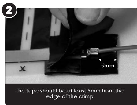
Place a piece of mastic on the underside of the crimp
